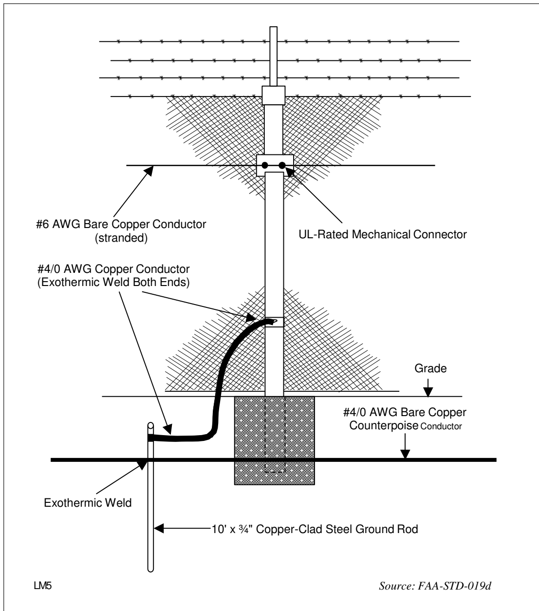
Figure 2-6. Grounding a Fence
